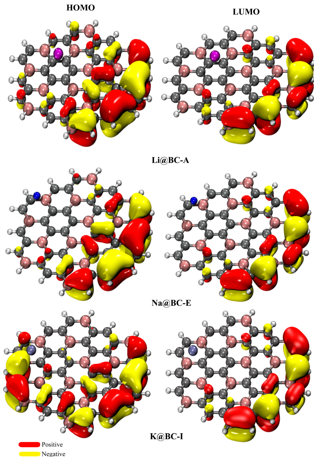
Fig. 2 HOMO and LUMO of M@BC nanosheets (Li@BN-A, Na@BC-E, K@BC-I).
