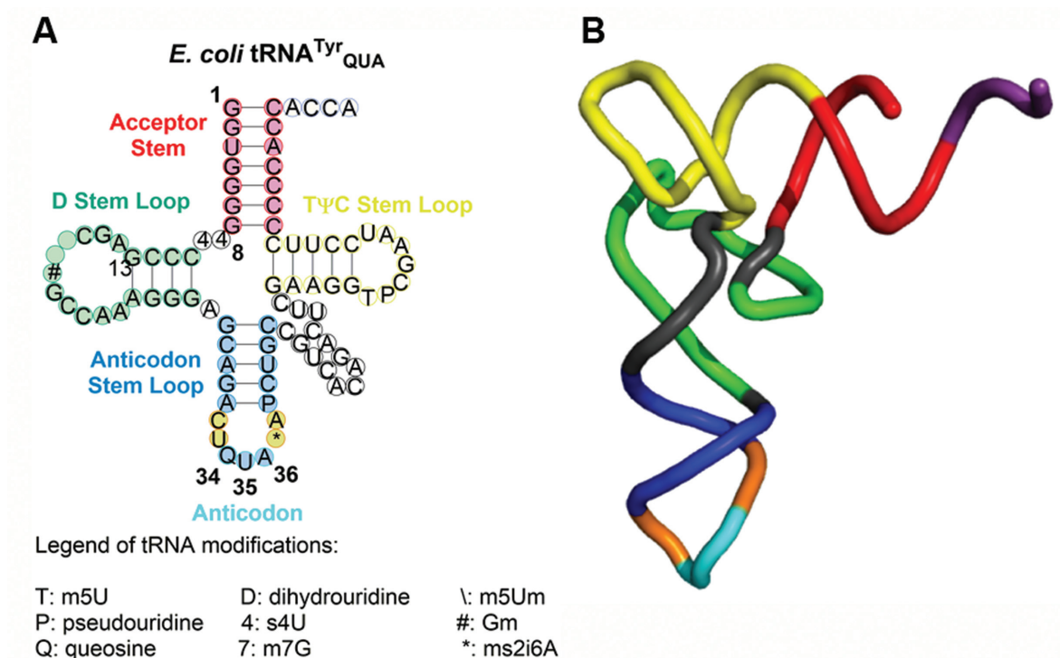
Figure 1. (A) Sequence and secondary structure of E. coli tyrosyl tRNA molecule. Modified nucleobases are indicated. (B) Backbone trace of tRNA structure (pdb 1EHZ), color coded to match secondary structural elements in (A).
