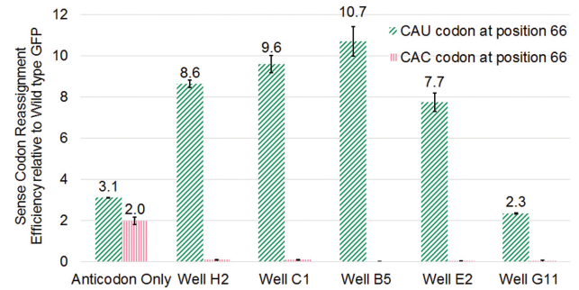
Figure 5. Codon discrimination for selected tRNA variants. Reassignment efficiencies reported as the observed optical density-corrected fluorescence divided by the optical density-corrected fluorescence of wild-type GFP for each orthogonal pair measured in response to CAU and CAC histidine codons specifying Y66 of GFP.
