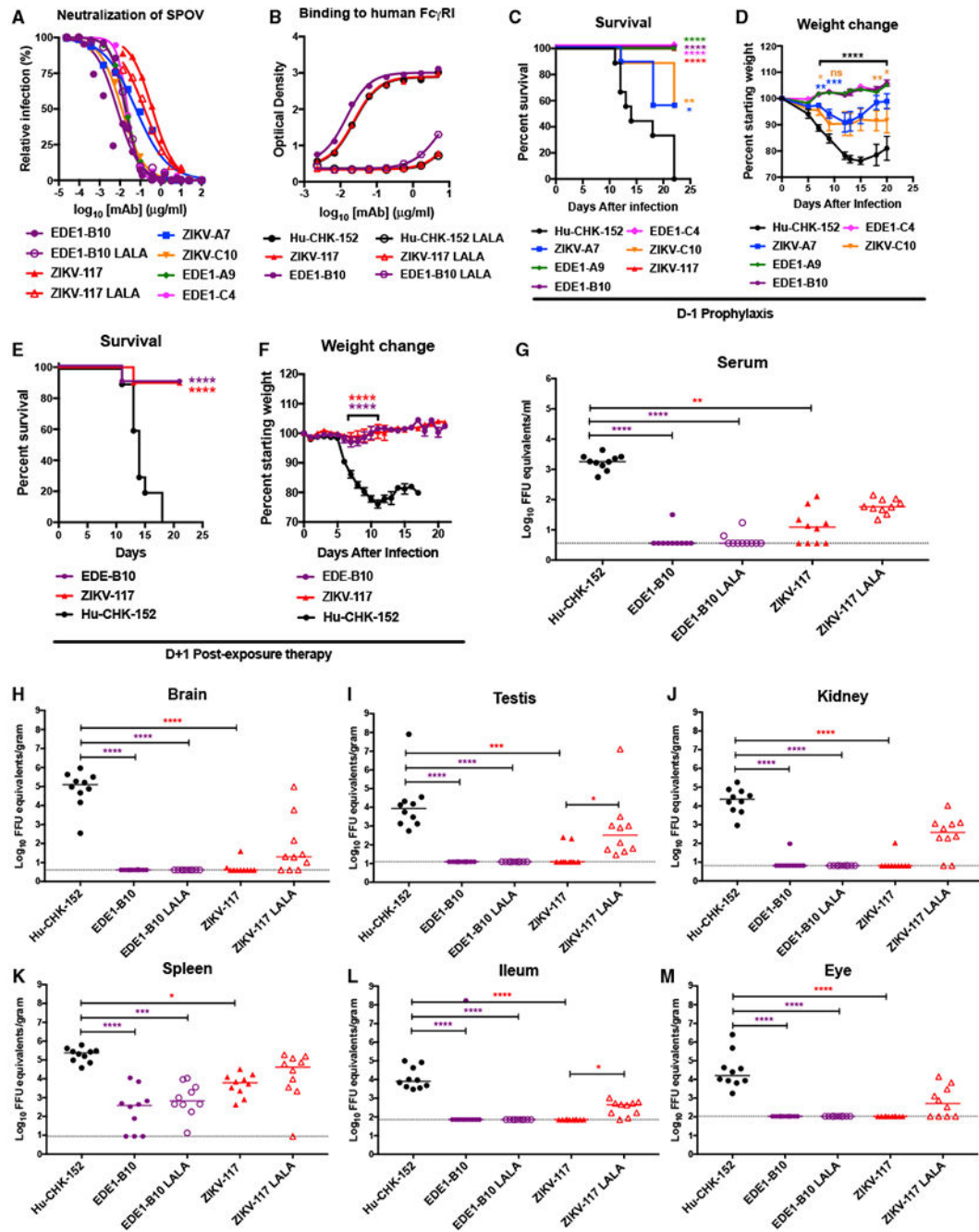
Figure 6. Neutralization and Protection against SPOV Infection by Cross-Reactive Anti-DENV or Anti-ZIKV mAbs
