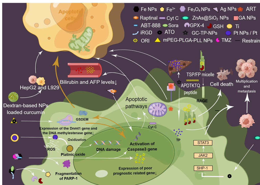
Figure 2 Schematic diagram of NPs and chemotherapy for HCC. NPs, nanoparticles. iRGD, Peptide chain of the amino acid sequence CRGDK/RGPD/EC. GSH, glutathione. PARP-1, poly (ADP-ribose) polymerase I. ABT-888, PARP-I inhibitor. Reprinted with permission from Figdraw ( www.figdraw.com ).
