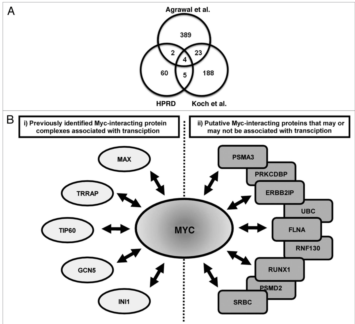
Figure 1. Expanding the Myc interactome. (A) Venn diagram comparing the known Myc interacting proteins (Human Protein Reference Database, HPRD) with recent publications using high-throughput mass spectrometry methods. (B) Schematic diagram representing several of the known Myc-interacting protein complexes and several of the putative interactors identified by Agrawal et al.
