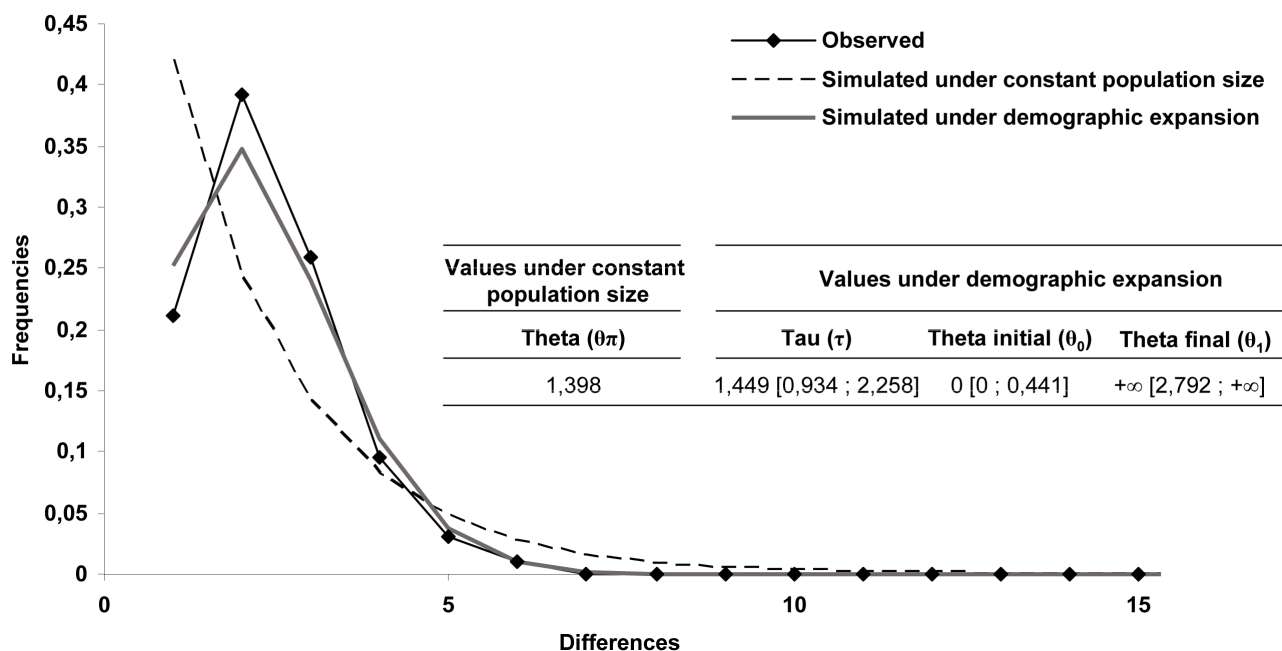
Figure 4. Mismatch distributions of COI haplotypes. COI haplotypes observed, simulated under a constant population size and a model of population expansion for the South-west Pacific populations of A. iwaotakii . Along x-axis are indicated the numbers of nucleotide differences between all pairs of sequences and on y-axis the frequencies of pairs. The table summarizes the parameters of demographic analyses under constant population size and demographic expansion. The confidence intervals at 99% of the parameters under a demographic expansion model are given in square brackets. doi:10.1371/journal.pone.0069680.g004
