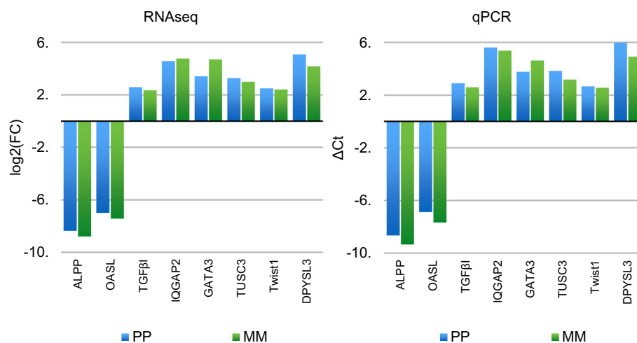
Fig. 6. Candidate gene verification using qPCR. Difference of crADSL against WT cells of biological quadruplicates in both PP and MM of RNAseq (A) and qPCR (B) were normalized to \beta -Actin. Expression patterns show consistency.
