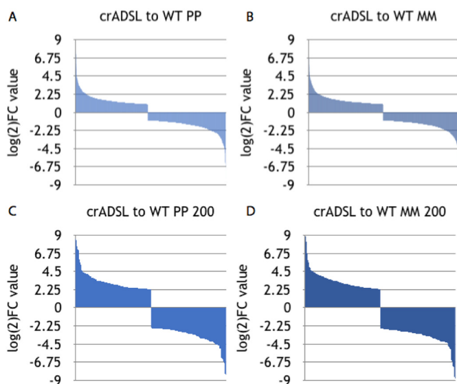
Fig. 4. \log_2 fold change of DEGs in cell lines under experimental conditions. A and B: all DEGs that satisfy cutoff constraints between PP comparison (A) and MM comparison (B). C and D: 100 most positively and 100 most negatively changed DEGs in PP comparison (C) and MM comparison (D).
