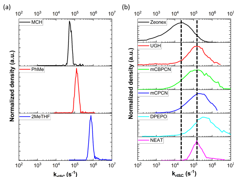
Figure 2. Distribution of k_{\text{rISC}} rates of (a) DMAC-TRZ in solvents of increasing polarity at 0.8 mM concentration and (b) 1% loading drop casted films of DMAC-TRZ in different hosts. All measurements were performed at room temperature. TRPL decay can be found in Figure S5.
