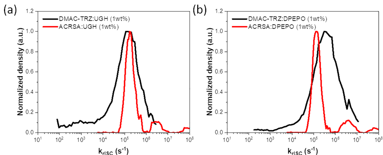
Figure 3. Comparison of the distribution of k_{\text{rISC}} rates between DMAC-TRZ and ACRSA in (a) UGH and (b) DPEPO, as a host matrix at 1% concentration. TRPL decay can be found in Figure S7.
