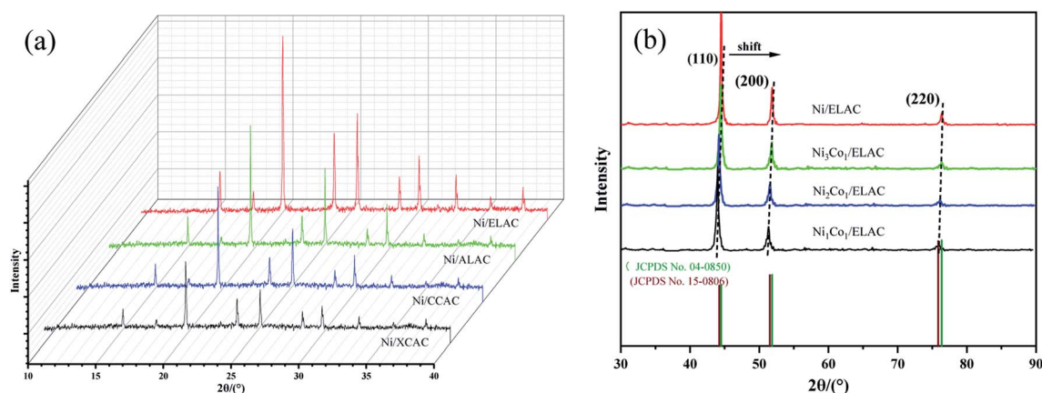
Fig. 1 XRD patterns of (a) Ni/ELAC, Ni/ALAC, Ni/CCAC and Ni/XCAC catalysts (b) Ni/ELAC, \text{Ni}_3\text{Co}_1/\text{ELAC} , \text{Ni}_2\text{Co}_1/\text{ELAC} , \text{Ni}_1\text{Co}_1/\text{ELAC} catalysts.
