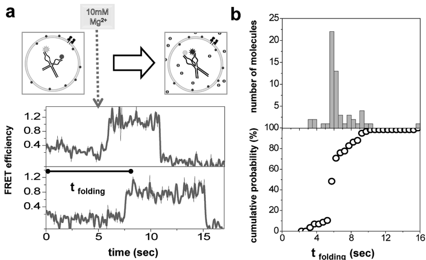
Figure 3. (a) At t = 0 , ribozymes encapsulated in porous SUVs are subject to no Mg^{2+} , hence stay unfolded (low FRET). Upon injection of 10 mM Mg^{2+} into the sample chamber (between fifth and sixth seconds after data acquisition, marked with a dashed arrow), ribozymes rapidly fold (transition to high FRET). The duration for the FRET value to reach \sim 0.8 from t = 0 is defined as time of folding ( t_{\text{folding}} ). The top and the bottom graphs belong to different SUVs (hence different ribozymes) from the same run (thin, black line: raw data; thick, gray line: B-spline smoothed data). (b) Histogram for times of folding (top) and corresponding percentile cumulative folding probability vs time (bottom) obtained from individual traces.
