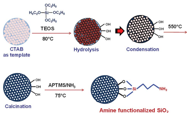
Scheme 1 Synthesis and functionalization of mesoporous silica nanoparticles.
