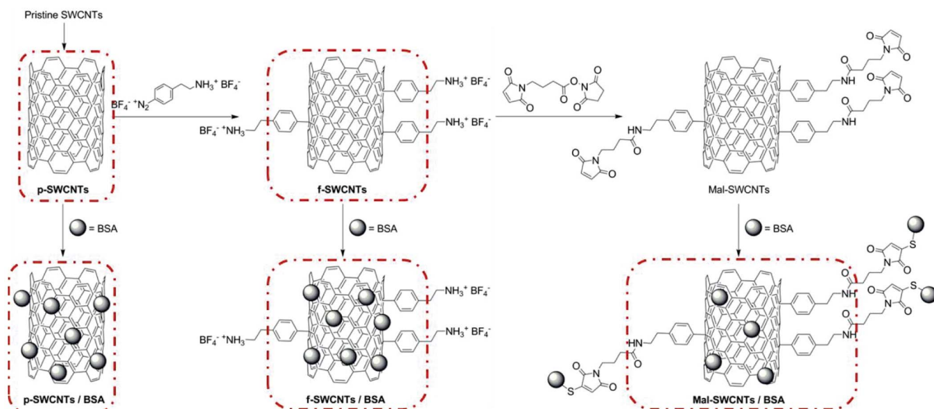
Figure 5 | Schematic of the purification and covalent functionalization of pristine SWCNTs. Boxes highlight the SWCNTs samples tested in this study. Figure adapted from Knyazev et al. 35 .
