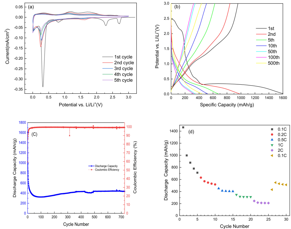
Figure 7. Electrochemical performance of MOA as anode material: (a) five first cyclic voltammograms recorded at 0.01 mV s -1 scanning rate, (b) galvanostatic charge/discharge curves carried out at 1C-rate (~1.1 A g -1 ) in the potential window 0.01–3.0 V vs. Li + /Li, (c) specific discharge capacity and Coulombic efficiency as a function of cycle numbers performed at a 1C-rate, and (d) rate capability.
