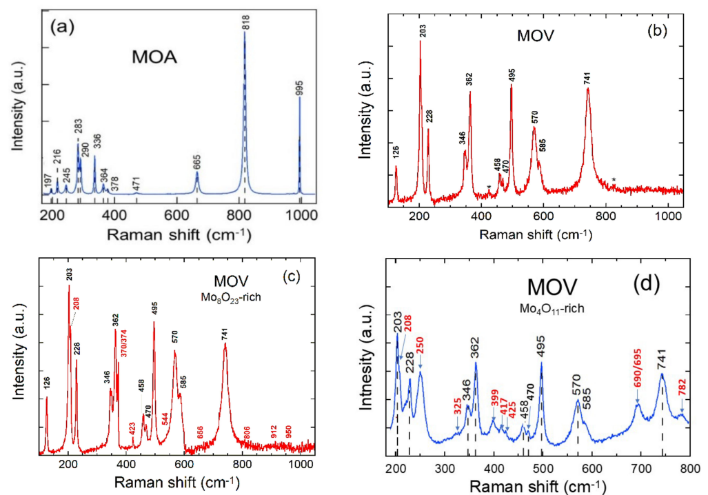
Figure 5. Raman spectra of the (a) MOA powders, (b) MOV ( \text{MoO}_2 -rich sample where the stars correspond to Raman peaks of suboxides), (c) MOV with m - \text{Mo}_8\text{O}_{23} -rich particles, and (d) MOV with o - \text{Mo}_4\text{O}_{11} -rich particles. Spectra were recorded at a spectral resolution of 1 \text{ cm}^{-1} .
