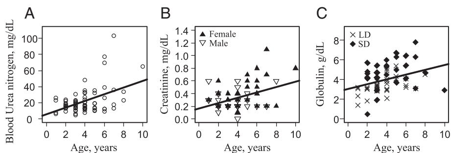
Figure 4 Statistical analyses were performed utilizing a Pearson correlation. (A) Simple linear regression between blood urea nitrogen levels and age ( n=77 , r=0.46 , p<0.001 ). (B) Simple linear regression between creatinine levels and age ( n=75 , r=0.28 , p<0.01 ). (C) Simple linear regression between total blood globulin concentration and age ( n=73 , r=0.20 , p<0.05 ), LD: long-day season; SD: short-day season.
