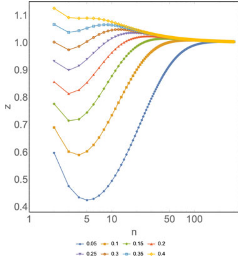
Fig. 1. z as a function of n for different prevalences ( x ) ranging from 0.05 to 0.4 for the particular case of New South Wales state, Australia. Horizontal axis: group size of a pooled sample ( n ). Vertical axis: number of tests per subject needed to diagnose one subject ( z ). Different colours represent different prevalences. Input: \varepsilon_1 = 0.101 , \varepsilon_2 = 0.691 , \varepsilon_3 = 0.208 , \gamma_1 = 0.396 , \gamma_2 = 0.941 and \gamma_3 = 1.489 .
