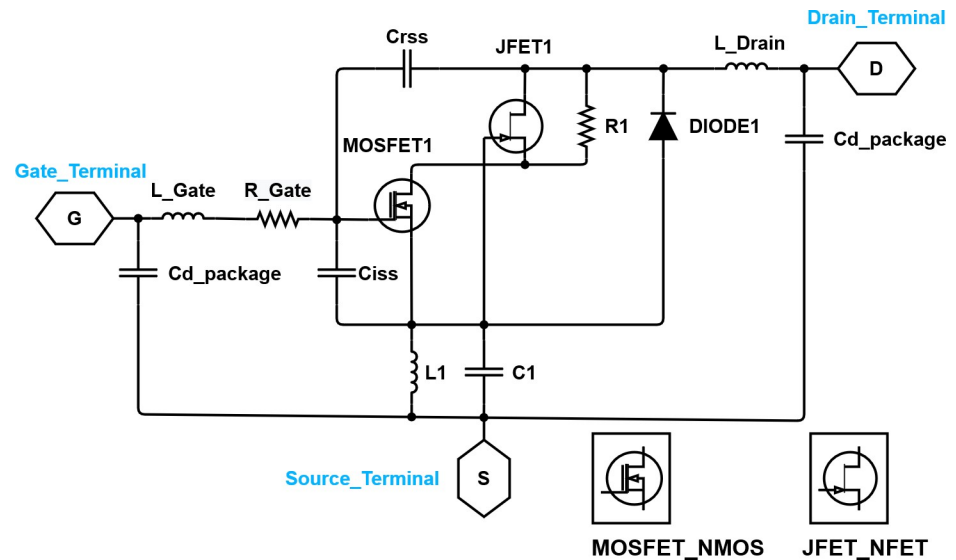
Fig 6. Large-signal LDMOSFET equivalent circuit provided by STMicroelectronics.
