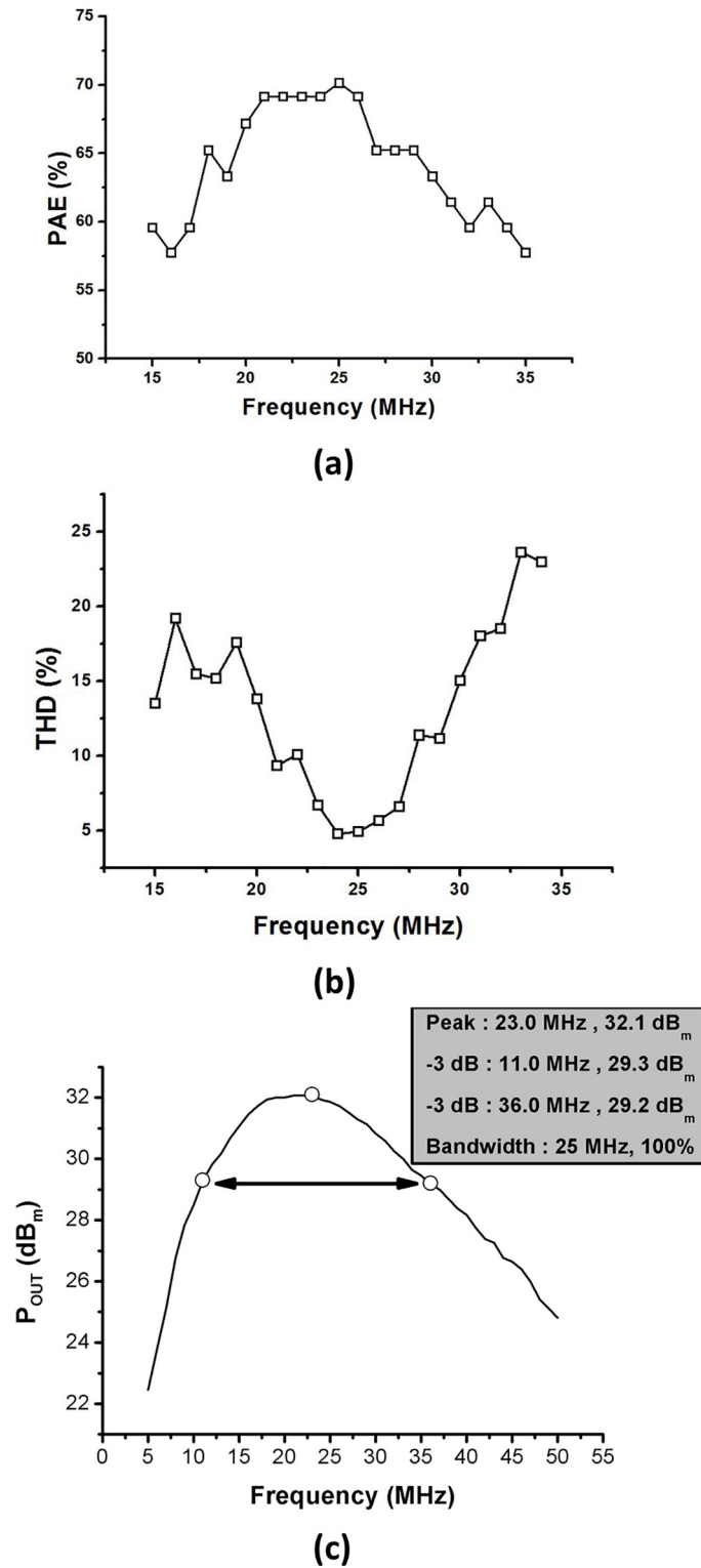
Fig 14. Curves showing variation of P OUT and calculated PAE and THD values obtained from high-efficiency and high-voltage class F amplifier with a 7.5 dBm input power according to frequency. (a) PAE vs. Frequency, (b) THD vs. Frequency, (c) P OUT vs. Frequency.
