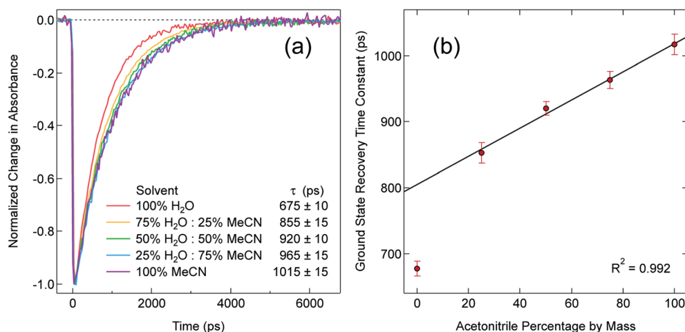
Fig. 8 (a) Time-resolved absorption data for ground-state recovery of [\text{Fe}(\text{bpy})_3]\text{Br}_2 in binary solvent mixtures of water ( \text{H}_2\text{O} ) and acetonitrile (MeCN) following ^1\text{A}_1 \rightarrow ^1\text{MLCT} excitation at 550 nm. (b) Fit of the time constants obtained from the data in part (a), showing a linear correlation between the kinetics of ground state recovery and the mass percentage of acetonitrile in the solvent mixture. The data point for pure water ( i.e. , 0% acetonitrile) was not included in the fit.
