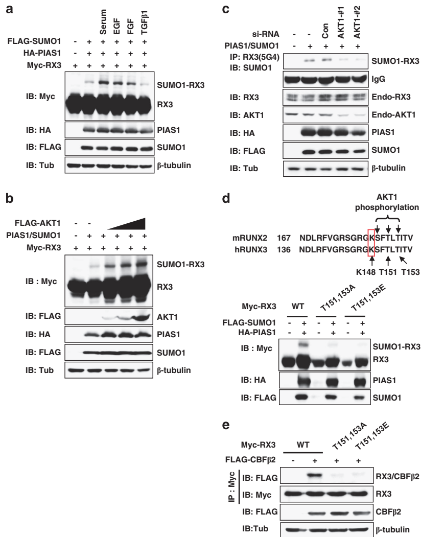
Figure 4. AKT1 stimulates RUNX3 sumoylation. (a) HEK293 cells were transfected with Myc-RUNX3, HA-PIAS1 and FLAG-SUMO1, and then serum starved for 24 h. Cells were then treated with serum, epidermal growth factor (EGF; 1 \mu g/ml), fibroblast growth factor (FGF; 30 ng/ml) or transforming growth factor- \beta 1 (TGF \beta 1; 5 nM) for 3 h. RUNX3 sumoylation was analyzed by IB. (b) Serially increasing levels of FLAG-AKT1 were coexpressed with Myc-RUNX3, HA-PIAS1 and FLAG-SUMO1 in HEK293 cells, and RUNX3 sumoylation was analyzed by IB. (c) HEK293 cells were transfected with HA-PIAS1 and FLAG-SUMO1 and treated with si-AKT1 (100 nM). Two independent si-AKT1 RNAs (#1 and #2) were used. Sumoylation of endogenous RUNX3 was detected by IP with anti-RUNX3 antibody (5G4) and IB with anti-FLAG antibody. (d) Amino-acid sequence around the RUNX3 sumoylation site (K148) was compared with that of RUNX2. The AKT1 phosphorylation sites of RUNX2 49 are indicated by arrows. The phosphorylation sites were mutated in RUNX3 to obtain RUNX3-T151,153A and RUNX3-T151,153E. RUNX3-WT, RUNX3-T151,153A or RUNX3-T151,153E was coexpressed with HA-PIAS1 and FLAG-SUMO1 in HEK293 cells, and RUNX3 sumoylation was analyzed by IB. (e) RUNX3-WT, RUNX3-T151,153A or RUNX3-T151,153E was coexpressed with FLAG-CBF \beta 2 in HEK293 cells, and the RUNX3-CBF \beta 2 interaction was analyzed by IP and IB.
