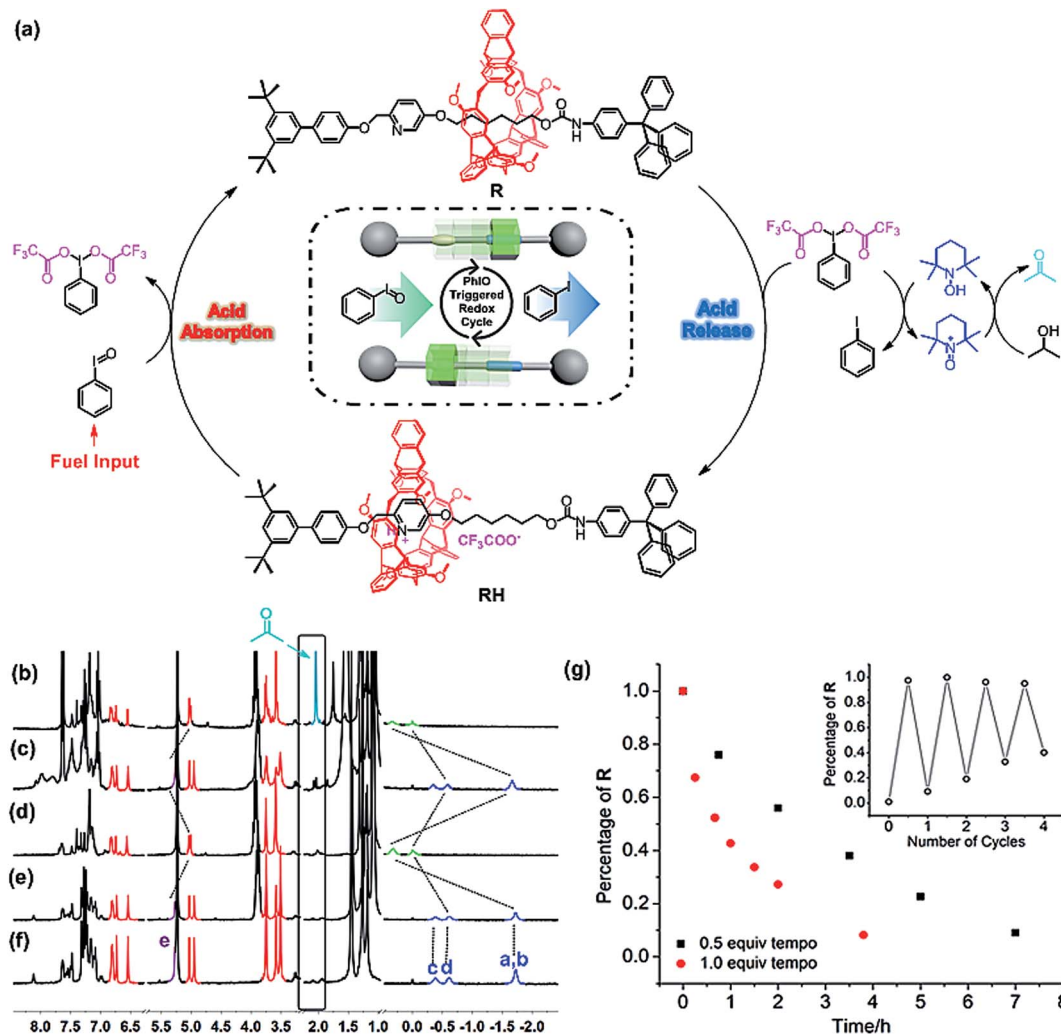
Fig. 3 (a) Mechanism and illustration of the chemical fueled switchable motion of the helicene-based [2]rotaxane powered by PhIO-triggered redox cycle; ^1\text{H} NMR spectra (300 MHz, \text{CD}_2\text{Cl}_2 , 298 K) of (f) R, (e) R + 0.5 equiv. of TEMPO + 25 equiv. of i -PrOH, (d) e + 2 equiv. of TFA, (c) d + 2 equiv. of PhIO, and (b) c after 7 h; and (g) kinetics of the mechanical movement controlled by different concentrations of TEMPO. Insert: reversible motion in the presence of 0.5 equiv. of TEMPO followed by the addition of the chemical fuel.
