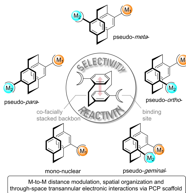
Figure 4. Heterobimetallic cyclophanyl complexes with varying M-to-M distances in spatial organization.
