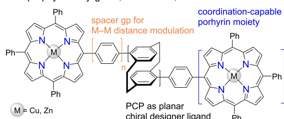
Figure 5. Model cyclophanyl complexes with varying M-to-M distances and coordination environments modulated via coordination-capable substituents
