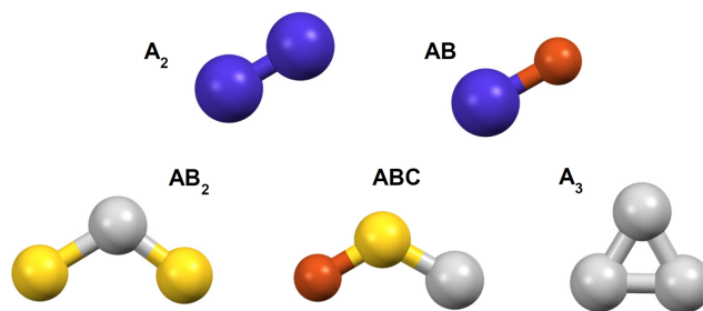
Figure 1. Types of metal combinations in complexes (reproduced from SFB/TRR 88 resources; Copyright 2018 3MET).
