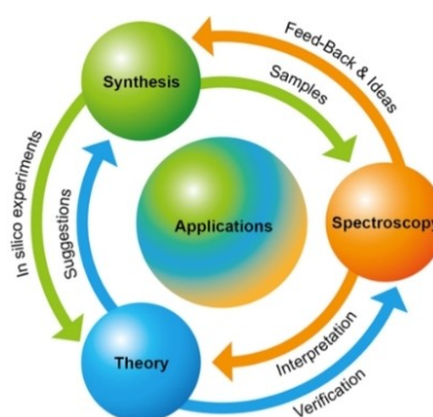
Figure 6. Cooperative research efforts by theoretical modeling, design/synthesis, and characterization of organometallic complexes (reproduced from SFB/TRR 88 resources; Copyright 2018 3MET).
