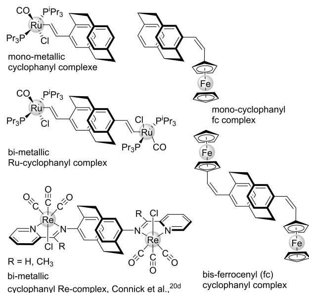
Figure 3. Electron delocalization via through-space and through-bond pathways in pseudo- para substituted cyclophanyl Ru, Re, and Fc complexes.
