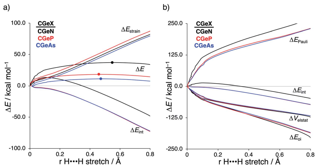
Fig. 4 (a) Activation strain analysis and (b) energy decomposition analysis of the \text{H}_2 bond activation by gerylenes CGeX with varying Group 15 ligands ( X = \text{NMe}_2, \text{PMe}_2, \text{AsMe}_2 ), where the transition states are indicated with a dot and the energies are projected onto the \text{H}\cdots\text{H} bond stretch of \text{H}_2 , computed at ZORA-BP86/TZ2P.
