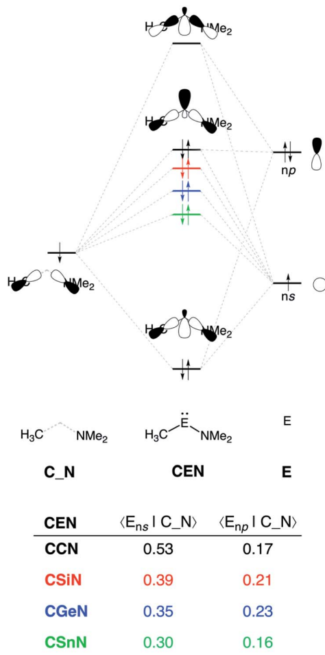
Fig. 3 Schematic representation of the construction of the CEN HOMO ( E = \text{C, Si, Ge, Sn} ) and orbital overlap between the atomic orbitals of E ( E_{ns} and E_{np} ) and the in-phase ligand orbital ( C\_N ), computed using ZORA-BP86/TZ2P level at consistent geometries with a \text{H}\cdots\text{H} bond stretch of 0.47 Å.
