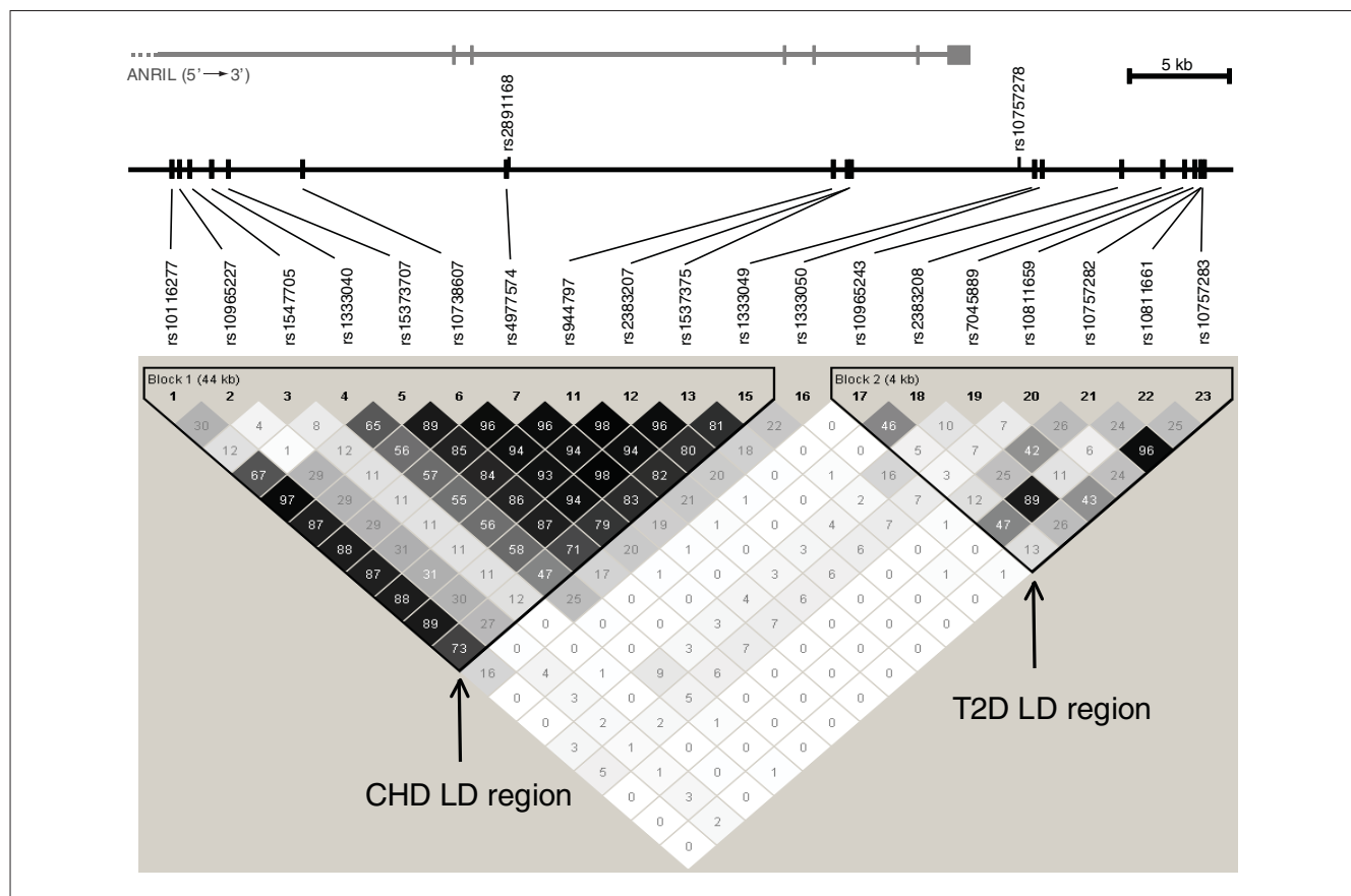
Figure 1 The pattern of LD in the European HGP samples on chromosome 9:22071397-22124172, a region approximately 53 kb long. R 2 values between each SNP pair are shown in shades of grey (black R 2 = 1, white R 2 = 0) and within each box. The CHD and T2D LD regions in Europeans are clearly separate. The SNPs best tagging the disease-associating haplotypes (rs4977574 and rs10811661) are in bold-face. The positions of two SNPs that have been identified as most strongly associated with CHD in two separate fine-mapping studies of Europeans, rs2891168 and rs10757278 (see text), are shown above the genomic sequence line. The position of the ANRIL gene is shown at the top, while the CDKN2B gene is located 72 kb upstream of the first SNP shown, rs10116277.
