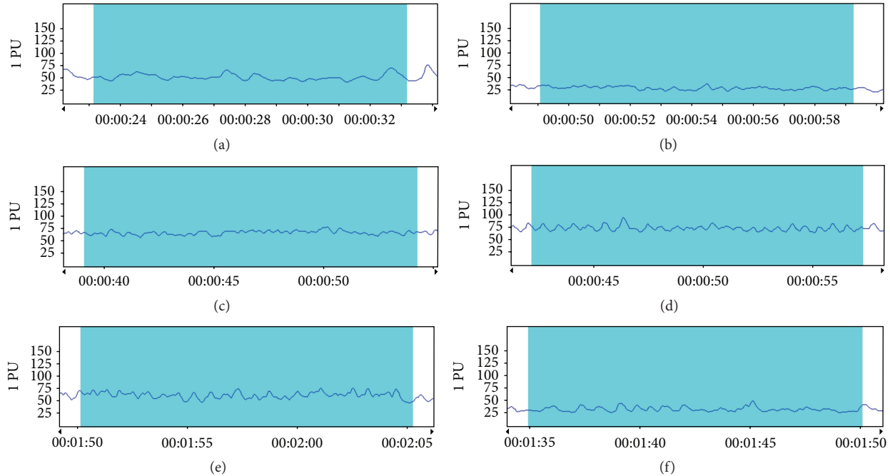
FIGURE 4: Representative blood perfusion curves of the pelvic microvessels. (a) The control group; (b) the model group; (c) the aspirin group; (d) the DZD-H group; (e) the DZD-M group; (f) the DZD-L group.
