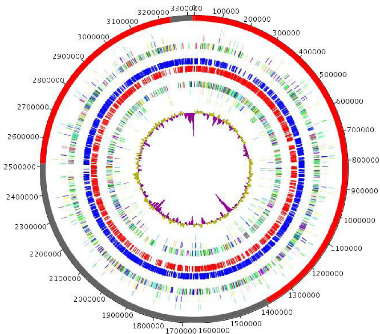
Figure 5. Graphical circular map of the A. massiliense strain JC14 T genome. From outside to the center: scaffolds (red / grey), COG category of genes on the forward strand (three circles), genes on the forward strand (blue circle), genes on the reverse strand (red circle), COG category on the reverse strand (three circles), G+C content.
