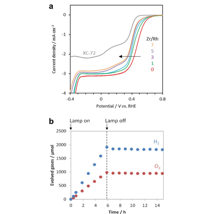
Fig. 12 (a) Current–potential curves of \text{RhZrO}_x (Zr/Rh: 0–7 w/w)-loaded carbon supports in \text{O}_2 -saturated 1 M \text{Na}_2\text{SO}_4 (pH 7); (b) gas evolution over time by \text{RhZrO}_x/\text{SrTiO}_3:\text{Al} (Rh = 0.1 wt% and Zr = 0.5 wt% vs. \text{SrTiO}_3:\text{Al} ) during and after light irradiation (300 W Xe lamp). Adapted with permission from ref. 169; copyright 2020 RSC.
