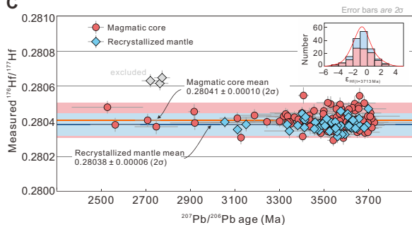
Fig. 2. Zircon structures, U-Pb ages, and Hf isotopic compositions of the Eoarchean Aktash tonalitic gneisses. (A) Representative CL images showing complex core (c), mantle (m), and rim (r) structures. Oscillatory zoned magmatic cores are surrounded by multiple recrystallized mantles that are separated by a thin bright seam (white arrows) with multiple metamorphic overgrowth rims. (B) Concordia diagram showing all U-Pb ages by secondary ion mass spectrometer (SIMS) and laser ablation (LA) (see Materials and Methods). The inset shows the ^{207}\text{Pb}/^{206}\text{Pb} ages of concordant analyses from magmatic cores and recrystallized mantles, with weighted mean ages of the oldest cores and youngest mantles interpreted as the best estimates of magma crystallization and metamorphic recrystallization, respectively. Other discordant analyses plot in the region defined by multiple radiogenic Pb ( \text{Pb}^* ) loss events. (C) Measured ^{176}\text{Hf}/^{177}\text{Hf} ratios versus ^{207}\text{Pb}/^{206}\text{Pb} ages for the magmatic cores and recrystallized mantles, showing the indistinguishable Hf isotopic compositions for both domains that do not change with apparent ages. The inset shows the near Gaussian distribution of \epsilon_{\text{Hf}} values calculated using the magmatic crystallization age.
