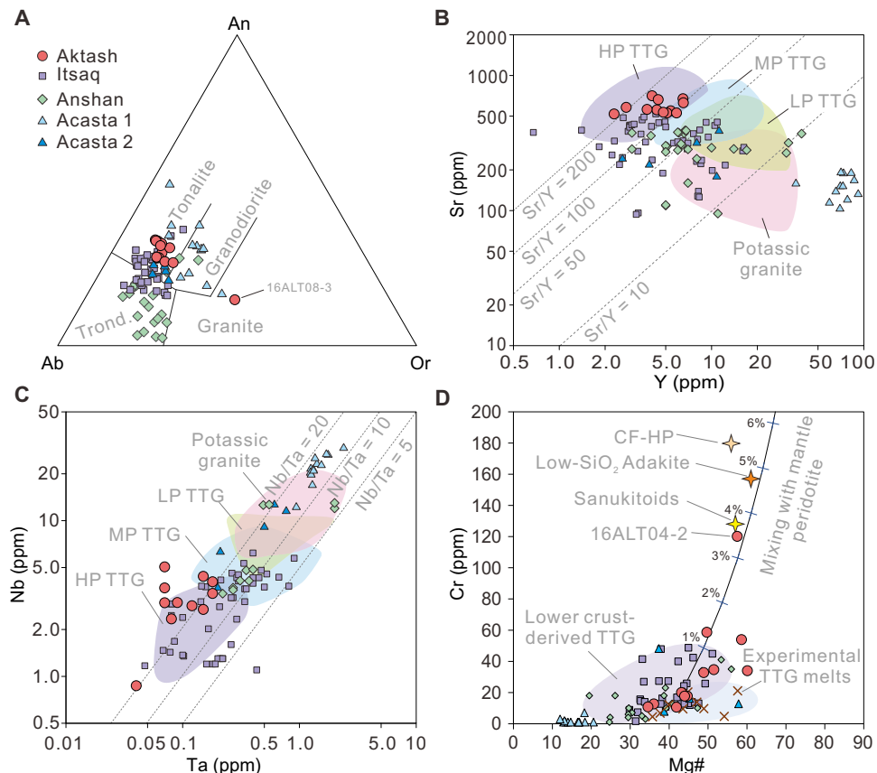
Fig. 3. Geochemical composition of the Eoarchean Aktash tonalitic gneisses compared to Eoarchean TTGs from the Itsaq, Acasta, and Anshan gneiss complexes. Average compositions of individual samples from replicate analyses are used in the plots for the Aktash gneisses. Acasta 1 refers to the 4.02-Ga high-FeO T tonalites that are compositionally different from typical TTGs. See table S4 for data source. (A) Feldspar triangular classification diagram showing the tonalitic composition of the studied samples, except for sample 16ALT08-3. (B) Sr/Y diagram. (C) Nb/Ta diagram. The Aktash tonalitic gneisses mostly plot into the HP TTG fields in (B) and (C), whereas other Eoarchean TTGs mostly plot into the medium and LP TTG fields (13). (D) Cr/Mg# diagram showing the higher Cr contents and Mg# of the Aktash tonalitic gneisses relative to the lower crust–derived Eoarchean TTGs and experimental TTG melts (37). The most “mafic” sample (16ALT04-2) plots close to the average low-SiO 2 Adakites and Archean Sanukitoids (3), which can be modeled by simple mixing with 3 to 5% mantle peridotite (DP1) (39). This provides a minimum constraint for mantle peridotite interacted with TTG melts because experiments show that this interaction produces peritectic mafic minerals (for example, garnet and pyroxene) that host most of the MgO, Cr, and Ni, so that even interaction with 30% peridotite produces melts (for example, CF-HP) similar to our most mafic sample (39).
