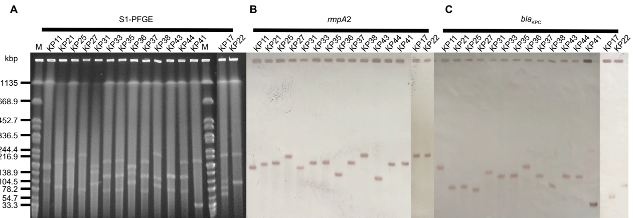
Figure 2 The S1-PFGE and Southern hybridization analysis of 15 Klebsiella pneumoniae strains co-harboring bla KPC-2 and rmpA2 .
