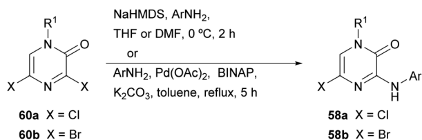
Scheme 17 Synthesis of 5-halo-2(1H)-pyrazinones 58 .
