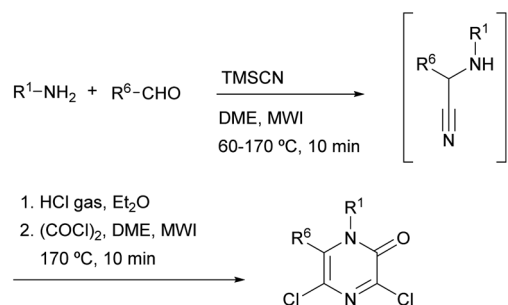
Scheme 15 Synthesis of 3,5-dichloro-2(1H)-pyrazinones under MWI.
