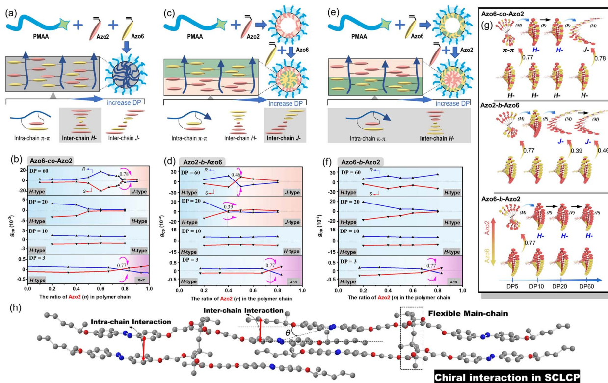
Fig. 3 Schematic representation of the PICSA procedure of (a) random Azo6-co-Azo2, (c) block Azo2-b-Azo6 and (e) block Azo6-b-Azo2 SCLCP assemblies. The g_{CD} values and the transition of stacking modes of (b) random Azo6-co-Azo2, (d) block Azo2-b-Azo6, (f) block Azo6-b-Azo2 SCLCP assemblies with the increase of DP and Azo2 ratios. (g) The internal stacking presented by the yellow Azo6 and red Azo2 units, respectively. (h) The homopolymer poly(Azo2) exhibits supramolecular polymorphism, and the unique asymmetric stacking modes can be depicted by the slip angle \theta according to Kasha's exciton theory. (dissymmetry factors, g_{CD} = \Delta\epsilon/\epsilon = [\text{ellipticity}/32\ 980]/\text{absorbance at the CD extremum} ).
