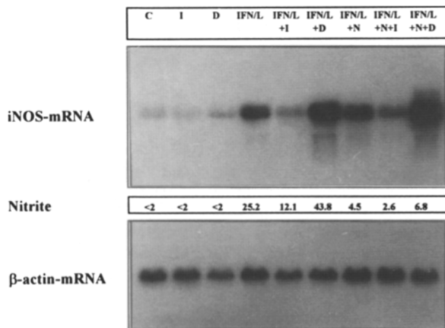
Figure 3. Modulation of mRNA levels for inducible NOS by \text{Fe}(3^+) , desferrioxamine, and \text{IFN-}\gamma/\text{LPS} . J774 cells were treated with ferric nitrate nonahydrate (I), desferrioxamine (D), NMA (N), and/or \text{IFN-}\gamma/\text{LPS} (IFN/L) for 20 h as described. Cellular mRNA was isolated and Northern blotting for inducible NOS mRNA and \beta -actin mRNA were carried out as detailed in Materials and Methods. Concentrations of nitrite ( \mu\text{mol/liter} ) in cell culture supernatants were determined by the Griess reaction (22) in order to ascertain whether modulations of cytoplasmic concentration of NOS mRNA by different treatments correlated with alterations of nitrite formation, used as a measure for NO production. One of three similar experiments is shown.
