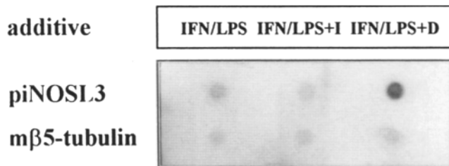
Figure 5. Modulation of inducible NOS gene transcription by iron and desferrioxamine. Nuclei of J774 cells treated with \text{IFN-}\gamma/\text{LPS} alone or in combination with 50 \mu\text{M} ferric nitrate nonahydrate (I) or 100 \mu\text{M} desferrioxamine (D) were prepared after 12 h of stimulation. Purification of nuclei and in vitro transcription were performed as described in Materials and Methods using the plasmid piNOSL3 and mβ5-tubulin. One of two similar experiments is shown. For densitometric evaluation of the runoff plots see Results.
