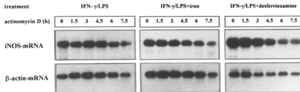
Figure 4. Effects of iron and desferrioxamine on NOS mRNA stability. In J774 cells, which were treated with ferric nitrate nonahydrate or desferrioxamine and \text{IFN-}\gamma/\text{LPS} for 20 h, transcription was inhibited by addition of actinomycin D ( 5 \mu\text{g/ml} ) for up to 7.5 h. Cells were harvested every 1.5 h after addition of actinomycin D. RNA was isolated and Northern blotting for NOS mRNA was carried out as described in Materials and Methods.
