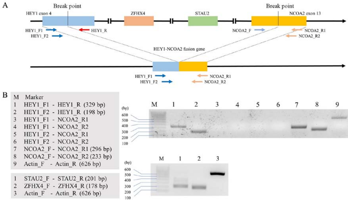
Figure 3. RT-PCR analysis of the HEY1-NCOA2 fusion. (A) HEY1 and NCOA2 gene structures. The upper panel displays the wild type. HEY1 and NCOA2 genes are located on chromosome 8q. The STAU2 and ZFXH4 genes are located between them. The lower panel displays previously reported fusion genes. (B) Results of RT-PCR. The fusion gene was not detected. The actin band was clearly evident. Normal NCOA2 , STAU2 and ZFX4F genes were detected. The results affirmed the absence of the fusion gene because those genes should be deleted if HEY1 and NCOA2 genes fuses at a certain breakpoint, and also indicated the success of RT-PCR. RT, reverse transcription; NCOA2 , nuclear receptor coactivator 2; STAU2 , staufen double-stranded RNA binding protein 2; ZFXH4 , zinc finger homeobox 4; HEY1 , hairy/enhancer-of-split related with YRPW motif 1.
