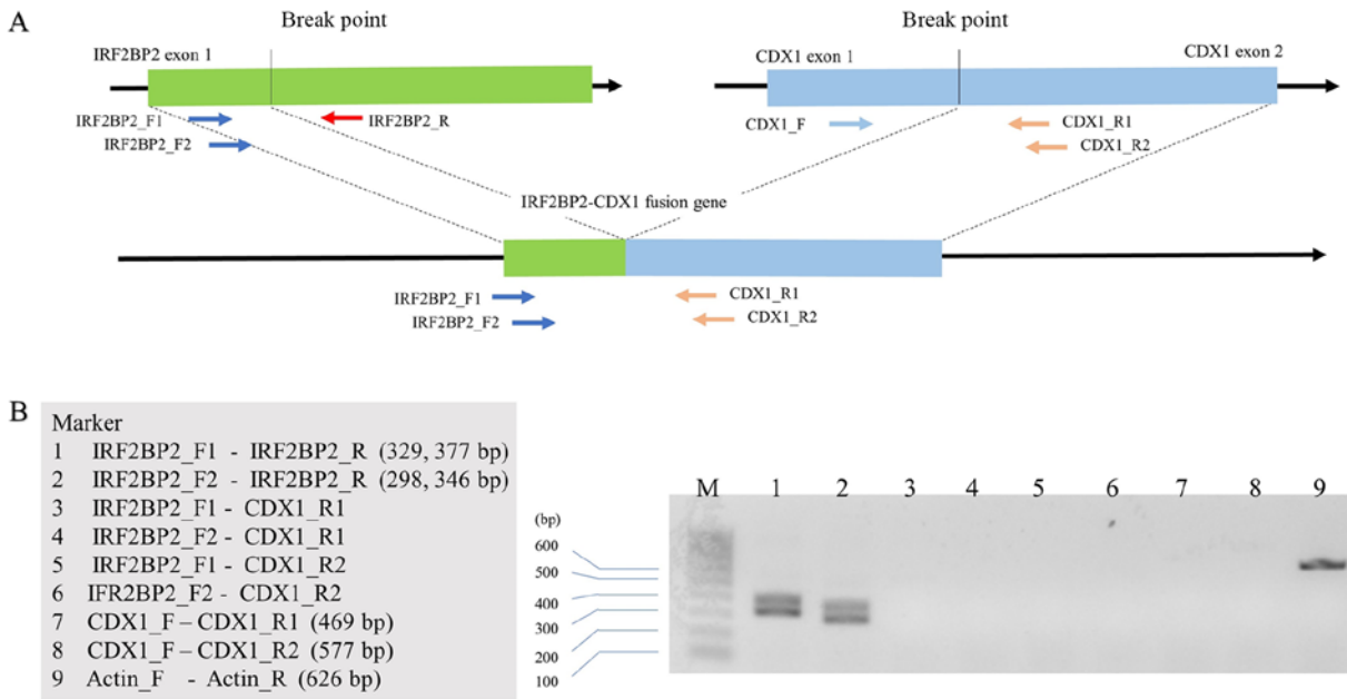
Figure 4. RT-PCR analysis of the IRF2BP2-CDX1 fusion. (A) IRF2BP2 and CDX1 gene structures. The upper panel displays the wild type. IRF2BP2 is located on chromosome 1q and CDX1 is located on chromosome 5q. The lower panel displays previously reported fusion genes. (B) Results of PCR. The IRF2BP2 and CDX1 gene fusion was not indicated, despite the presence of the actin band. Normal IRF2BP2 gene was detected as double bands reflecting its two isoforms. Normal CDX1 was difficult to detect with RT-PCR possibly due to GC richness in the CDX1 sequence. RT, reverse transcription; IRF2BP2 , interferon regulatory factor 2 binding protein 2; CDX1 , caudal type homeobox 1.
