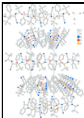
Fig. 2. Unit cell packing of (I) viewed down the b -axis. Dotted lines indicate hydrogen bonds.
