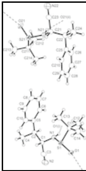
Fig. 1. A view of the two molecules in the asymmetric unit of (I). Displacement ellipsoids are drawn at the 50% probability level. Symmetry operations, (i): x-1/2, -y+3/2, -z ; (ii): -x, y+1/2, -z+1/2 .
