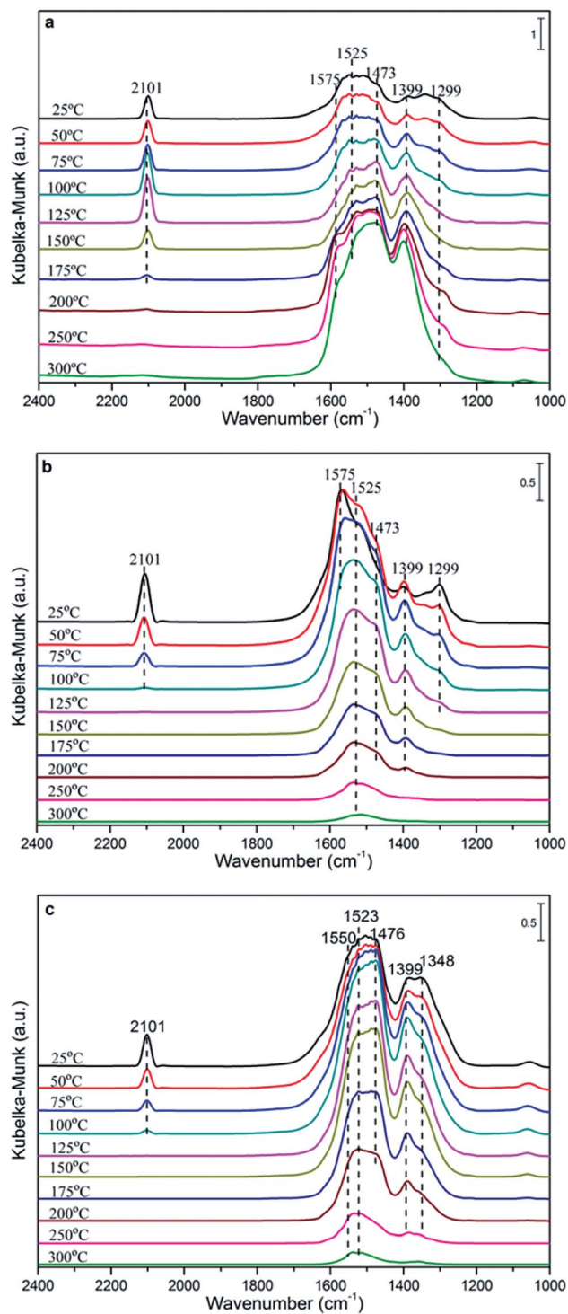
Fig. 8 DRIFTS spectra recorded after exposure to CO on the \text{Cu}_{0.1}\text{Ce} sample (a) and CO + \text{O}_2 on the \text{Cu}_{0.1}\text{Ce} (b) and \text{Cu}_{0.2}\text{Ce} (c) samples at different temperatures.
