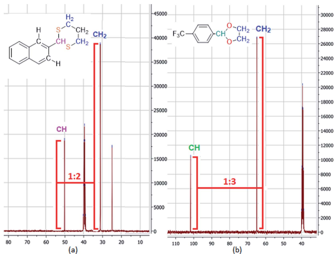
Fig. 4 Comparing NOE effect in 13 C-NMR spectrum of products. ((a) Part of 13 C-NMR spectrum of 2-(naphthalen-2-yl)-1,3-dithiane (1c). (b) Part of 13 C-NMR spectrum of 4CF 3 -2-phenyl-1,3-dioxolane (2h)).
