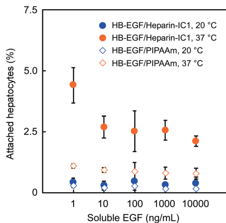
Fig. 4 Inhibitory attachment of rat hepatocytes to HB-EGF/heparin-IC1 and HB-EGF/PIPAAm surfaces after 1.5 h incubation with soluble EGF in serum-free DMEM containing 2 \text{ mg mL}^{-1} BSA. Seeding density, 5 \times 10^4 cells per \text{cm}^2 . The plots and error bars represent the mean and SD of triplicate experiments.
