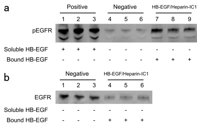
Fig. 5 Phosphorylated EGFR of rat hepatocytes cultured on HB-EGF/heparin-IC1 surfaces after 1.5 h incubation in serum-free DMEM containing 2 \text{ mg mL}^{-1} BSA. Hepatocyte lysates were analysed in triplicate by western blotting with (a) anti-phospho EGFR and (b) anti-EGFR antibodies. Negative and positive represented the suspension of hepatocytes stimulated without or with 1 \mu\text{g mL}^{-1} soluble HB-EGF for 15 min at 37^\circ\text{C} , respectively.
