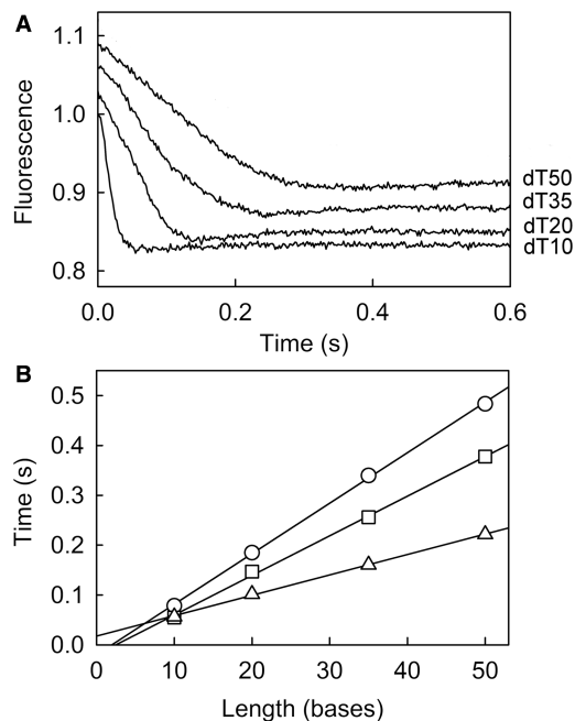
Figure 2. Translocation of MDCC-PcrA along ssDNA. (A) MDCC-PcrA was premixed with different lengths of oligo(dT), then rapidly mixed with ATP in the solution conditions (buffer and temperature, 22°C) of the TIRF measurements. The time to minimum fluorescence for each length represents the time for the last PcrA molecules to translocate to the 5'-end. The curves are offset from each other for clarity. (B) These time were plotted against length (squares) to give the translocation rate of 125 (\pm 2) \text{ bases s}^{-1} from the gradient. These plots are also shown for measurements under the conditions used by Dillingham et al. (21) for translocation (circles, 20°C, 50 mM Tris-HCl, pH 7.5, 150 mM KCl and 3 mM MgCl 2 ), giving 99 (\pm 2) \text{ bases s}^{-1} , and the solution plasmid unwinding conditions of Slatter et al. (14) (triangles, 30°C, 50 mM Tris-HCl, pH 7.5, 100 mM KCl, 10 mM MgCl 2 and 1 mM EDTA), giving 244 (\pm 4) \text{ bases s}^{-1} .
