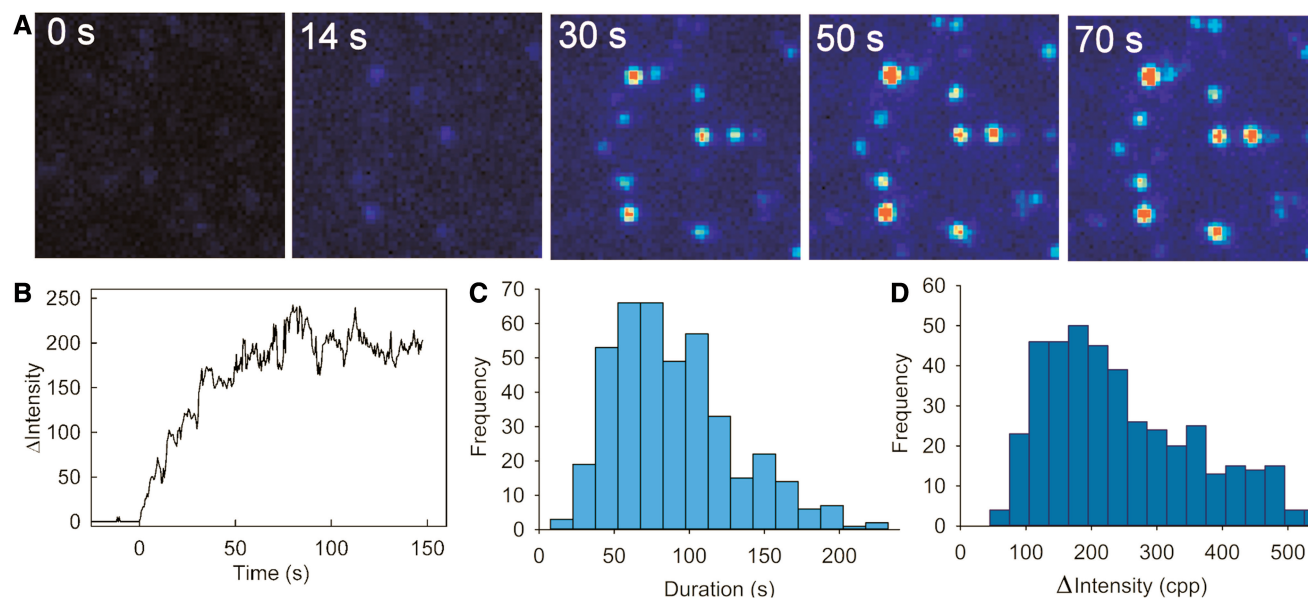
Figure 7. Visualization of circular plasmid DNA unwinding using immobilized PcrA. Cy3B-bioPcrA was used together with RepD and 3094-bp plasmid; see ‘Materials and Methods’ section for details. Zero time was set as the time of the start of the unwinding event. (A) Visualization of individual fluorescent spots of increasing intensity with time on an area of 25\mu\text{m}^2 . (B) Representative example of time course. (C) Distribution of event durations for one experiment (414 events). The average duration is 83 (\pm 2) s, giving a rate of unwinding of 41 (\pm 1) \text{s}^{-1} for this set of events, assuming complete unwinding. (D) Distribution of event intensity changes. The data from this set of measurements are summarized in Table 2.
