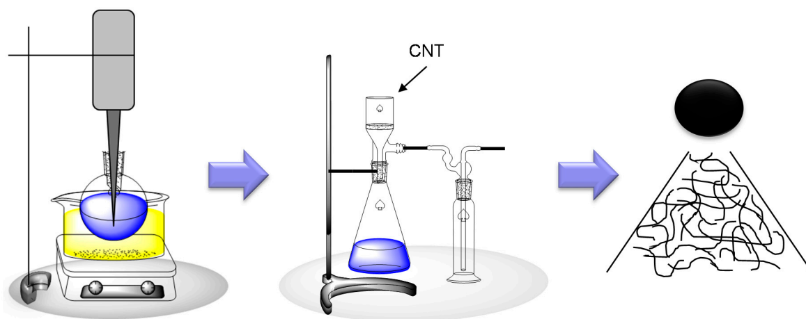
Figure 4. Scheme of CNT buckypaper preparation; tip-sonication ( left ), filtration under lower pressure ( middle ), resulting buckypaper ( right ).
