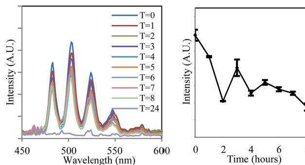
Fig. 2 The decrease in the intensity of uranyl emission over time in the steady-state emission spectrum of anaerobic uranyl solutions containing Geobacter sulfurreducens ( \lambda_{\text{ex}} = 420 \text{ nm} , 77 K).
