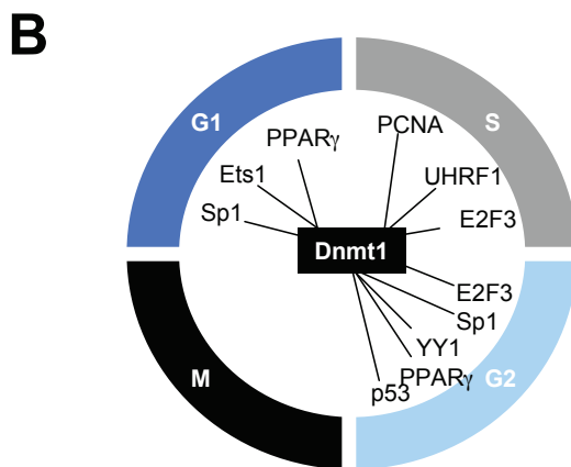
Figure 2 Dynamic of the formation and of the recruitment on DNA of the Dnmt1/transcription factor-including complexes during the cell cycle. (A) Graph (mean \pm SEM) illustrating the number of Dnmt1/transcription factor dots per nucleus in U251 cells during the different phases of the cell cycle. The number of Dnmt1/transcription factor interactions is calculated from the analysis of, at least, 50 nucleus in three independent experimentations. (B) Schematic representation of the dynamic of the Dnmt1-including complexes during the cell cycle.
