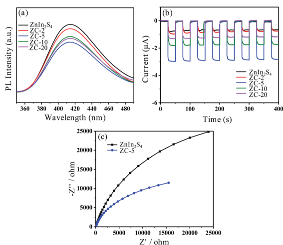
Fig. 5 Photo-luminescence (PL) spectra of \text{ZnIn}_2\text{S}_4 and prepared ZC- X composites (a) photocurrent–time curves of \text{ZnIn}_2\text{S}_4 and prepared ZC- X composites under the irradiation of simulated sunlight (b) Nyquist impedance plots of EIS for \text{ZnIn}_2\text{S}_4 and ZC-5 (c).
