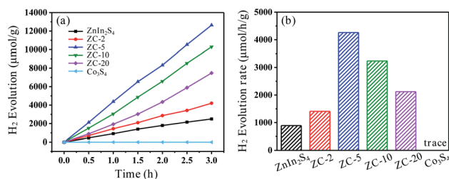
Fig. 6 The photocatalytic \text{H}_2 evolution performance over the synthesized \text{ZnIn}_2\text{S}_4 and ZC- X composites (a) the photocatalytic \text{H}_2 evolution rate of prepared \text{ZnIn}_2\text{S}_4 and ZC- X composite photocatalysts (b).
