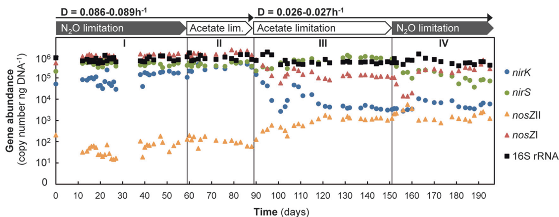
Fig. 1 Abundances of 16S rRNA, nosZI , nosZII , nirS , and nirK genes during operation of the N_2O -reducing chemostat under four conditions (I–IV) with either acetate or N_2O as growth-limiting factor, under two different dilution rates (D)
