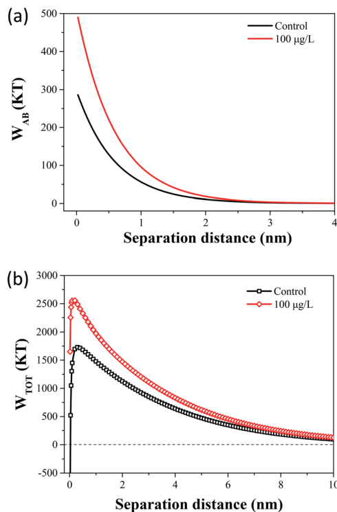
Fig. 6 (a) The effect of 100 µg L -1 TCS on W_{AB} in the prediction of XDLVO. (b) Total interaction energy profile as a function of particle distance with the prediction of the XDLVO theory.
