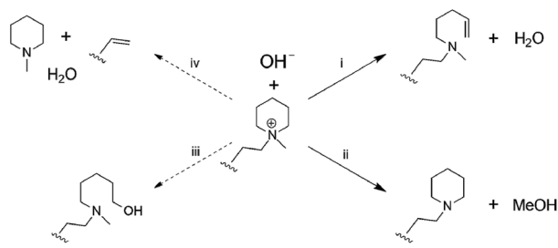
Fig. 13 Possible hydroxide ion induced degradation mechanisms of the piperidinium end-capped alkyl spacers. (i) Ring opening Hofmann-elimination, (ii) demethylation, (iii) S N 2 of hydroxide ion, and (iv) chain scission of alkyl spacer via Hofmann-elimination.
