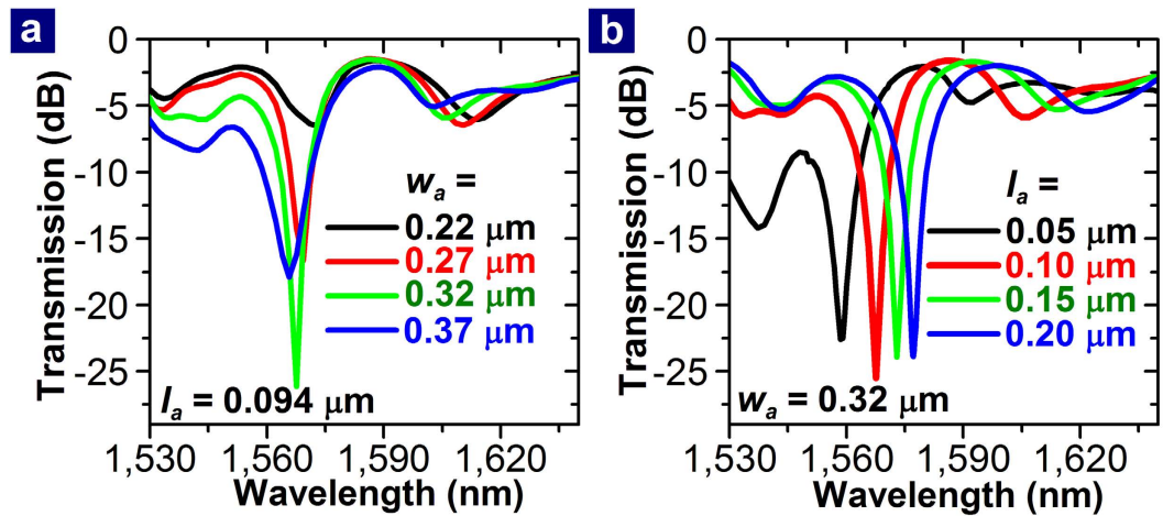
Figure 6. Dependence of the transmission spectrum on w_a and I_a . The transmission spectra of the MISIM waveguide with w_s = 50 nm which is coupled to the PDR with r_D = 0.9 \mu\text{m} are shown for various values of (a) w_a and (b) I_a .
