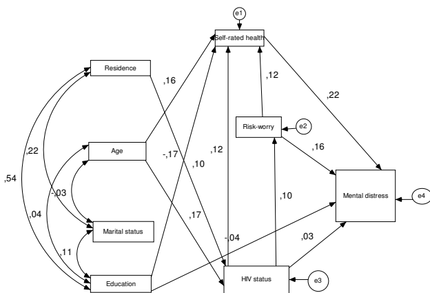
Path diagram of structural equation model
