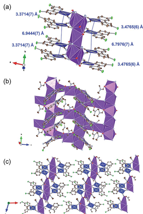
Fig. 2 (a) Stacking structure, (b) packing structure around \text{K}^+ ion and (c) crystal packing of 1·0.75DMF . Hydrogen atoms are omitted for clarity. Gray, light blue, red, and green ellipsoids show the C, N, Cl, and O atoms, respectively. The blue and purple polyhedra indicate Pt and K centers, respectively. Displacement parameters are drawn at 50% probability level. These pictures were illustrated using the VESTA computer program. 47
