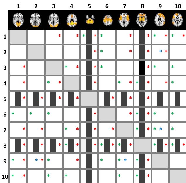
Fig. 5. Comparison of the effects of hallucinogenic drugs on between-network connectivity obtained by another group (Carhart-Harris et al., 2016b; Roseman et al., 2014) and our results. All results on networks identified in the present study were included. Asterisks indicate significant differences between drug and placebo condition (green: Roseman et al., 2014; blue: Carhart-Harris et al., 2016b; red: present study). Black indicates networks which were not investigated. Roseman et al. reported separate results for two representation of the DMN, which were combined in this presentation. (For interpretation of the references to color in this figure legend, the reader is referred to the online version of this chapter.)
