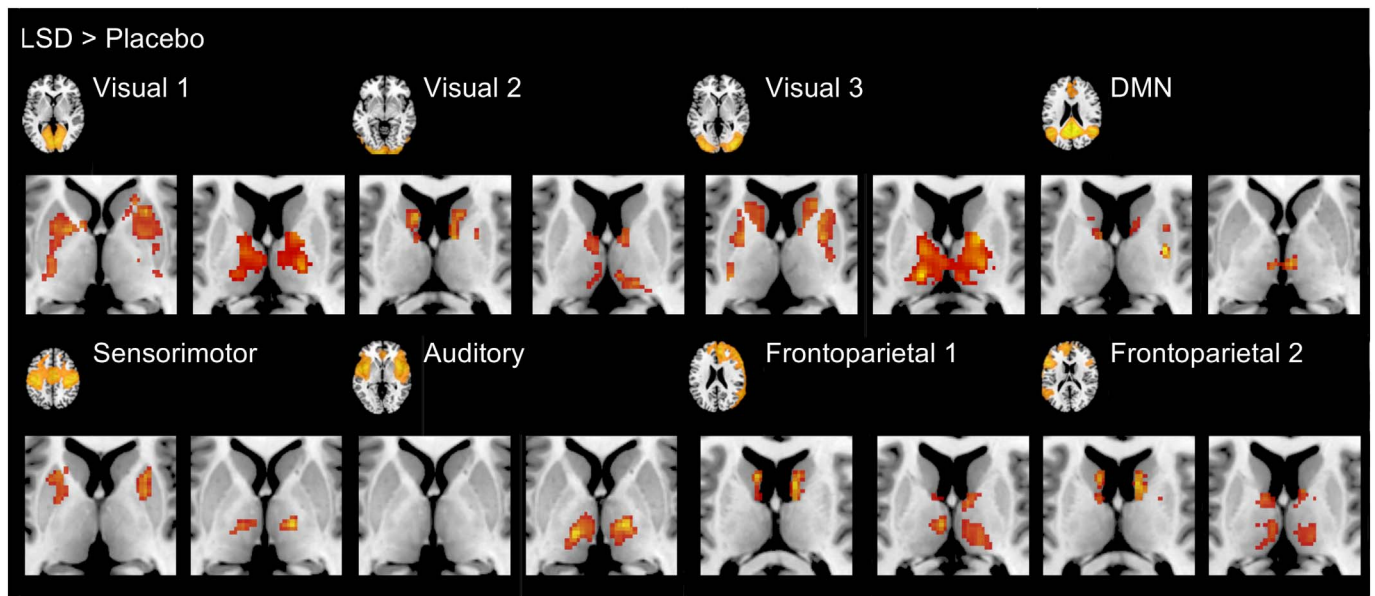
Fig. 4. Functional projections of resting state networks on striatal (left) and thalamic (right) structures. Only increases in FC were observed (cluster threshold p < 0.005 , FDR, two tailed, cluster-forming threshold p < 0.001 ). Right is right side of the brain.
