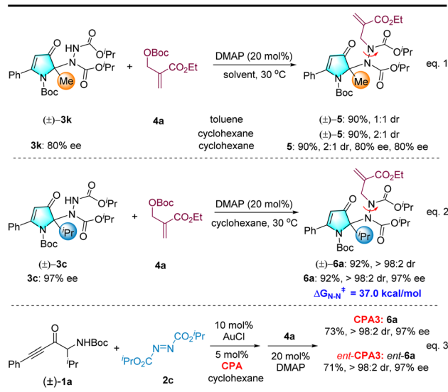
Scheme 4 Investigation of axially chiral hydrazide and the effect of CPA.
