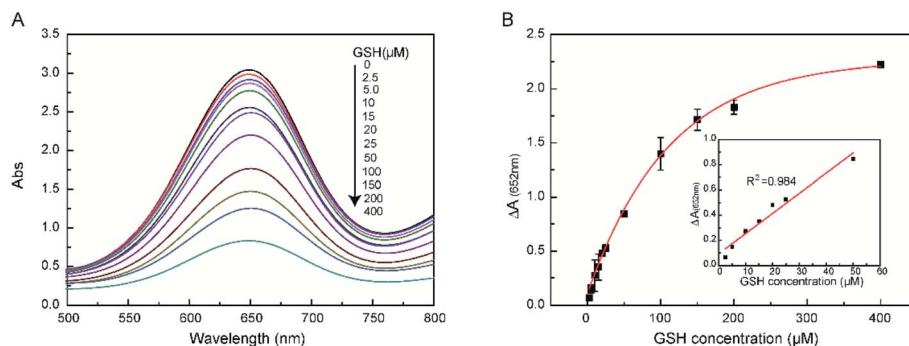
Fig. 4 (A) Changes in absorbance for TMB catalyzed by CNPs in the absence or presence of GSH (pH = 4.0). (B) Dose–response plot for GSH measurement. \Delta A = A_0 - A_{\text{max}} , where A_0 is the absorbance of the catalytic reaction for CNPs and A_{\text{max}} is the absorbance with GSH at 652 nm. The inset shows a linear curve for GSH.
