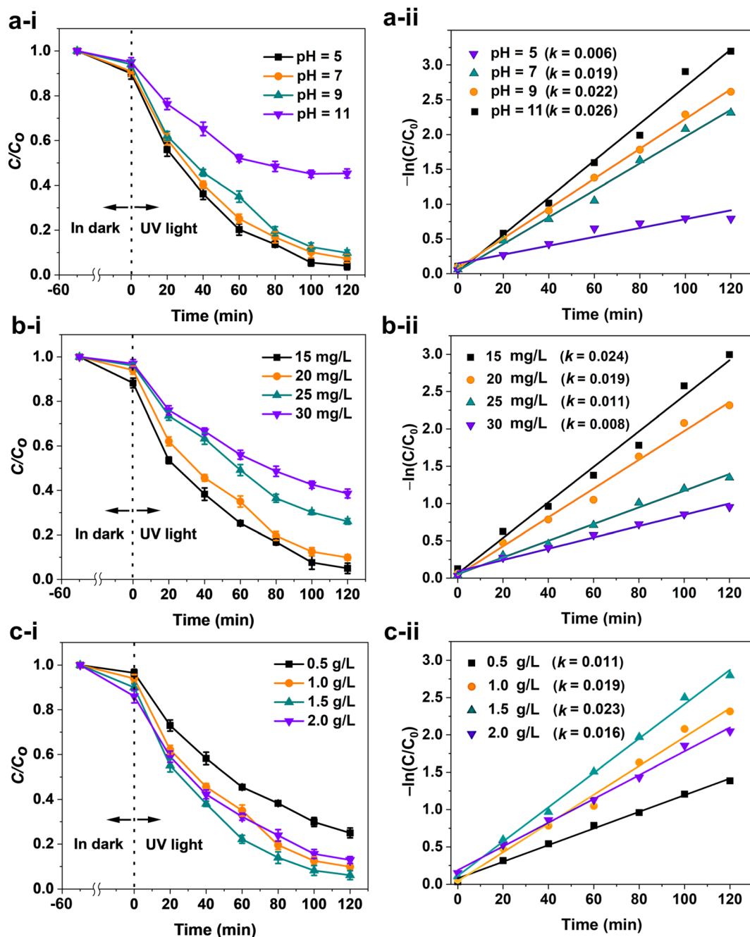
Fig. 9 Dependent graphs of C/C_0 vs. time (i) and their corresponding first-order plots (ii) for the degradation of RB5 dye by the ZIF-8-F3 material under UV irradiation in three different explorations: (a) initial pH, (b) initial RB5 concentration, and (c) used ZIF-8-F3 catalyst dosage.
